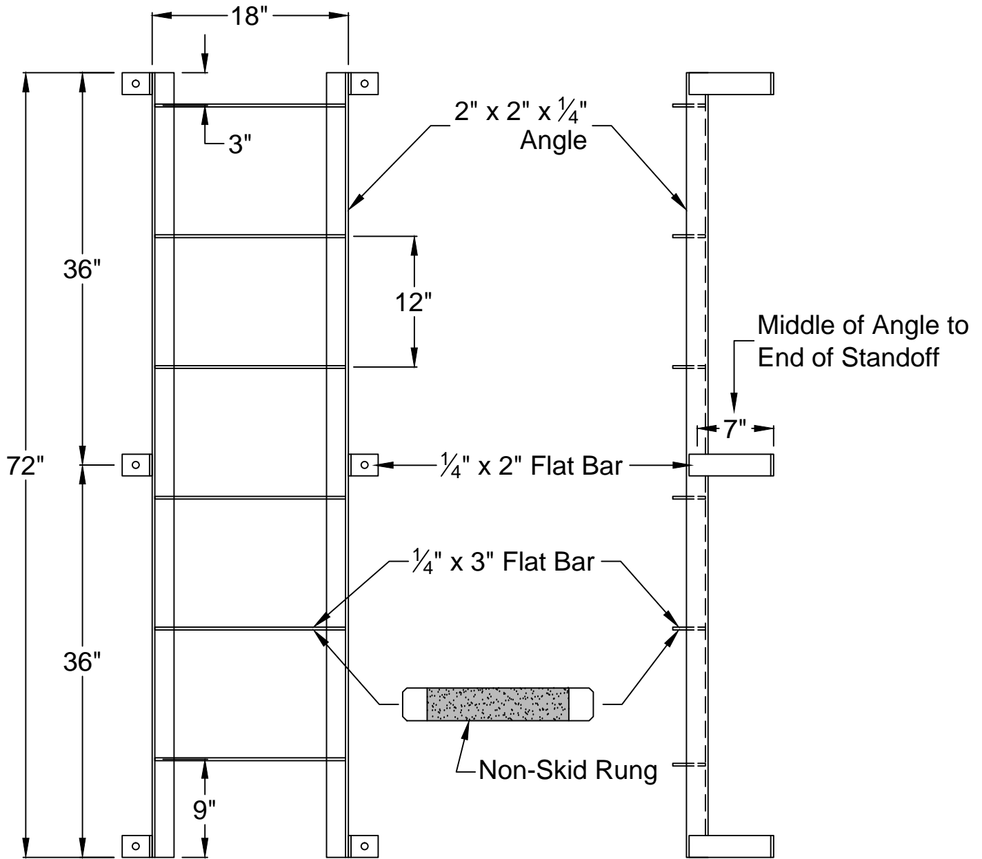
Side Elevation
