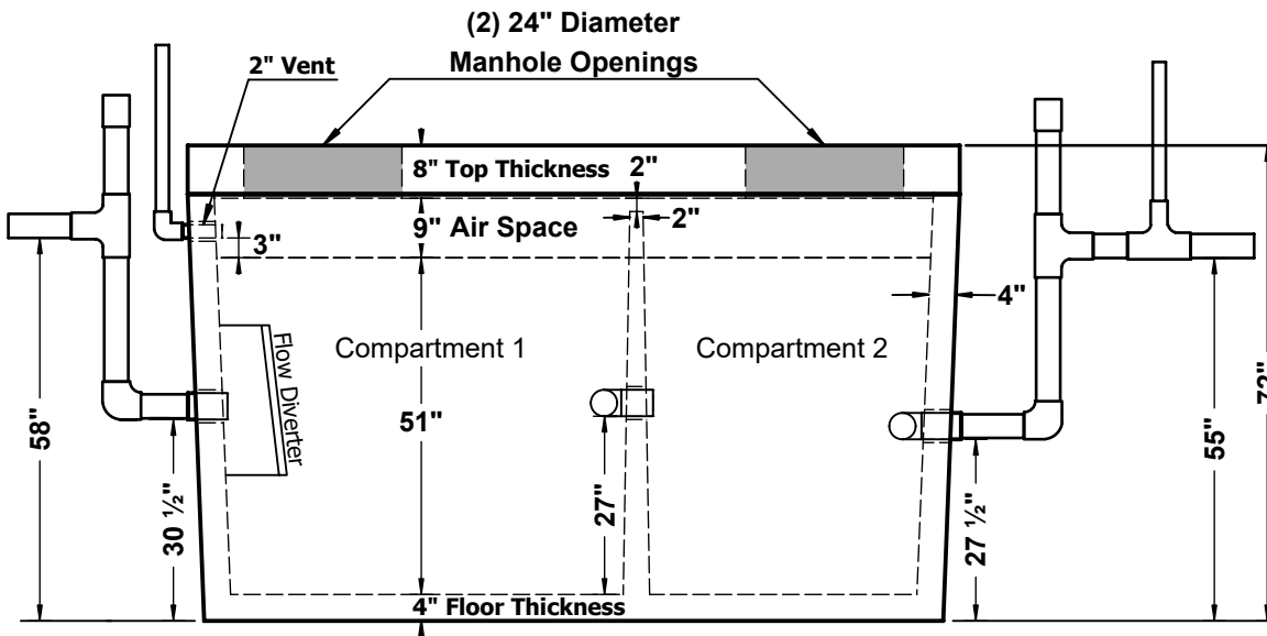
Profile View
